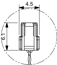
DETAIL C SCALE 3:1
